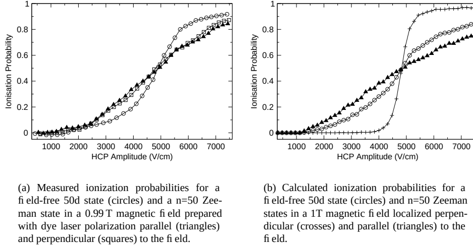
Figure 1.9: Measured and calculated ionization probabilities for a field-free 50d state and a n=50 Zeeman state in a 0.99 T magnetic field.
