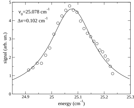
Figure 6.6: Measured absorption line profile of the \text{H}_2\text{O} ( J, K_a, K_c ) = (2 1 1) \leftarrow (2 0 2) transition (open circles). The line represents a Voigt profile fit to the data. The x-axis is converted from field to wavenumber using Fig. 6.1c.
