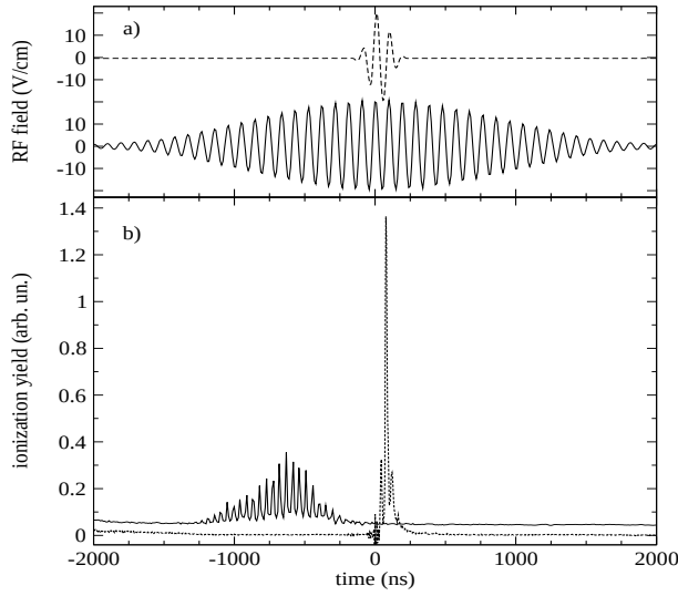
Figure 2.6: a) 10 MHz RF pulses with equal amplitudes of 21.5 V/cm and durations of 95 ns (dashed) resp. 1.2 \mu s (solid). b) Electron emission of a 90d state subjected to the RF pulses in a). The traces are set off vertically for clarity.
